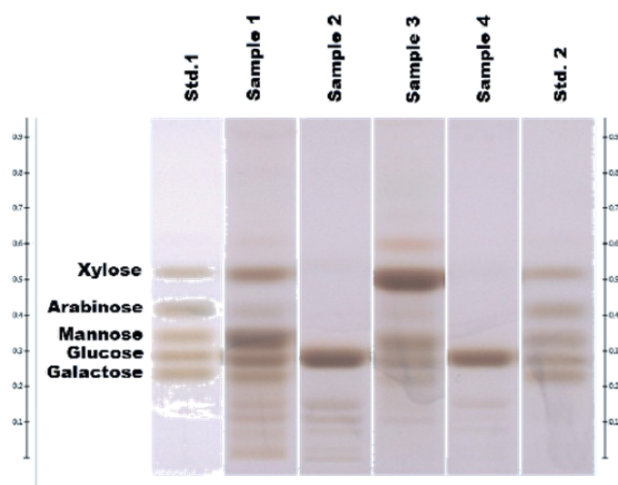
HPTLC chromatogram of wood-hydrolyzate sugars
