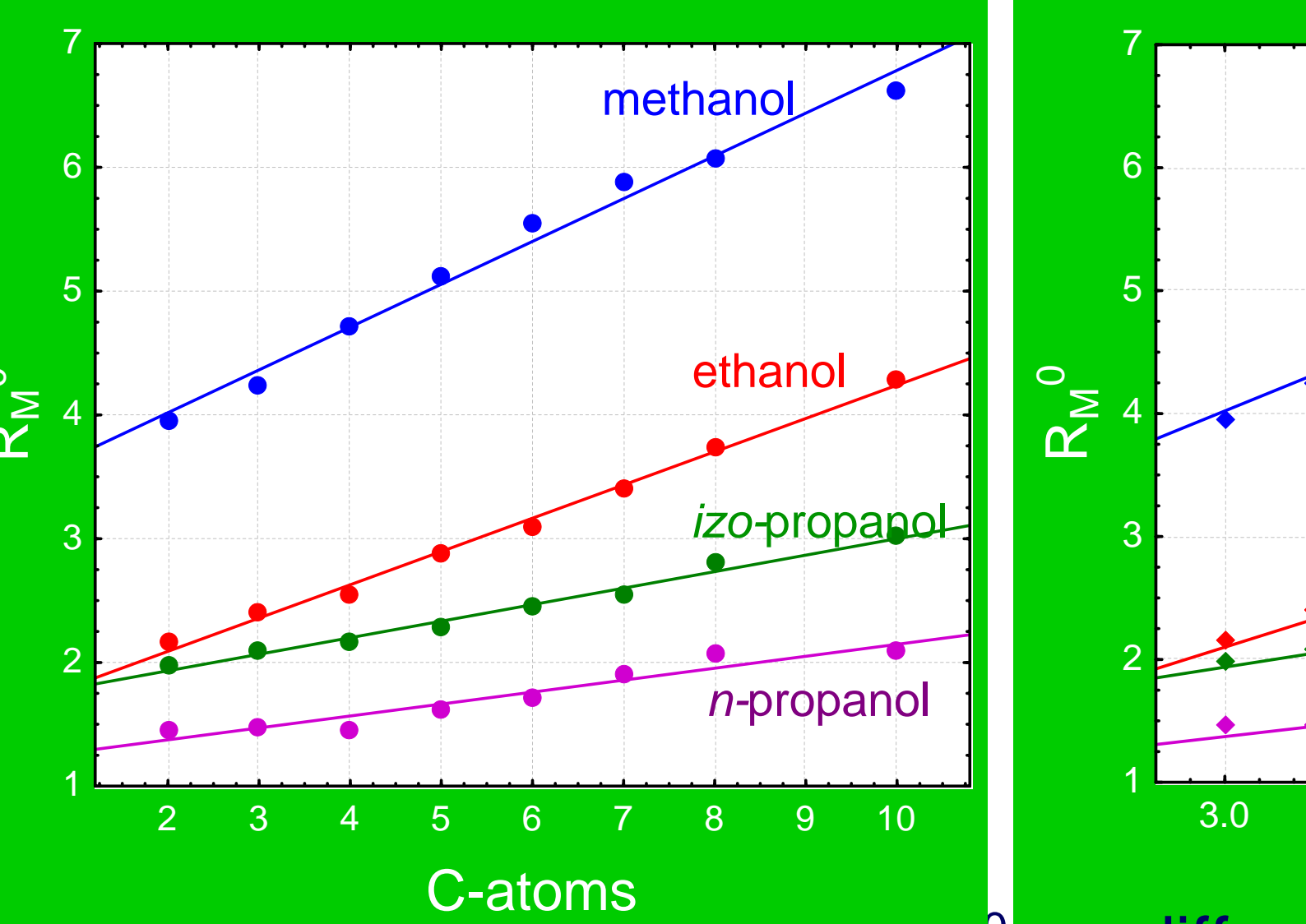
Figure 1. Chromatographic R_M^0 vs. different conclusions atoms, \log P , water solubility
